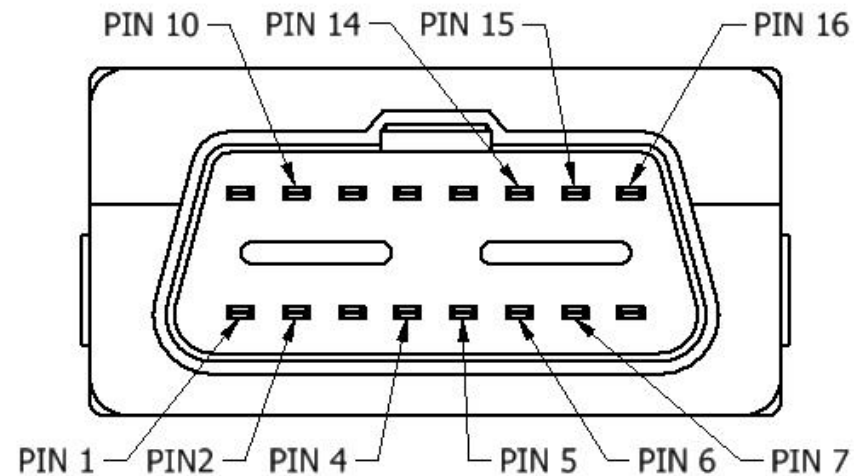
Figure 2 FMB001 OBDII socket pinout
