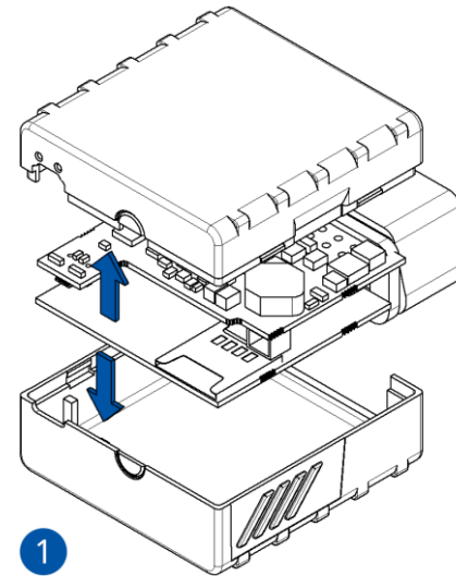
Figure 3 Cover removal
