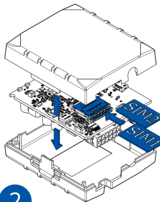
Figure 5 SIM card insert
