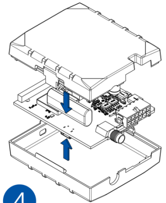
Figure 7 Attaching cover back
