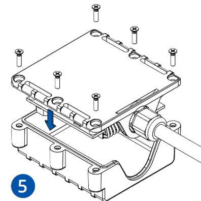
Figure 8 Attaching cover back
