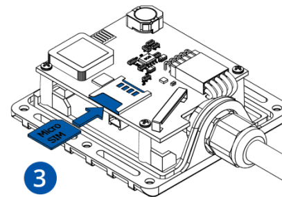
Figure 6 Micro-SIM card insert
