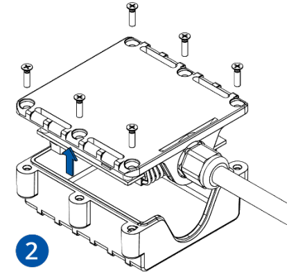
Figure 5 Cover removal
