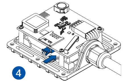
Figure 7 Battery connection
