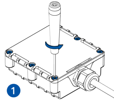
Figure 4 Unscrew screws
